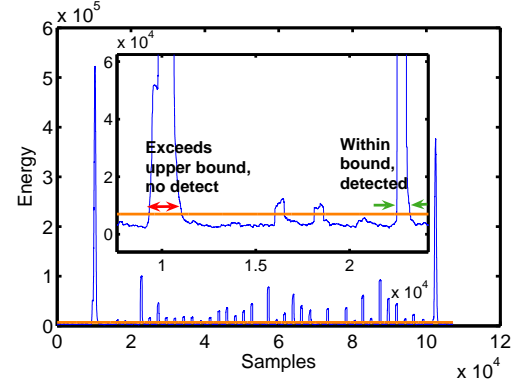
Fig. 6. Energy levels of footstep data at each time window
