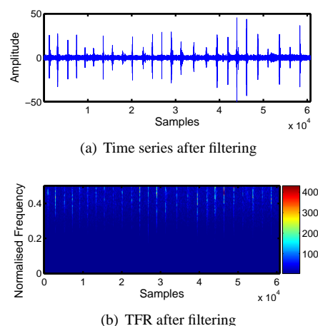
Fig. 5. Filtered footstep data from walking in boots on concrete at 2 feet from sensor
