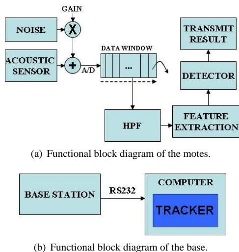
Fig. 3. Schematic block diagram of functional units.
